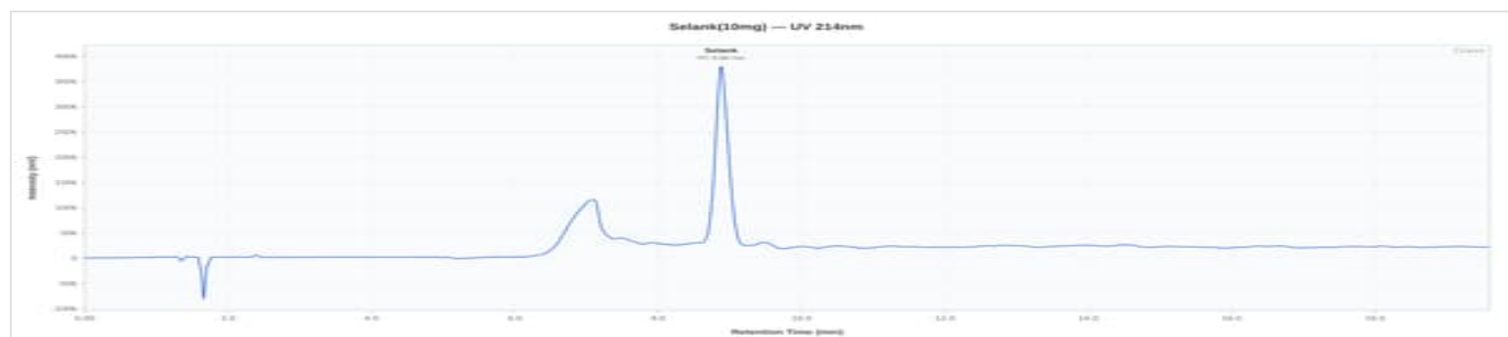
Selank 10mg - NS-SELANK-10MG: UV Chromatogram
