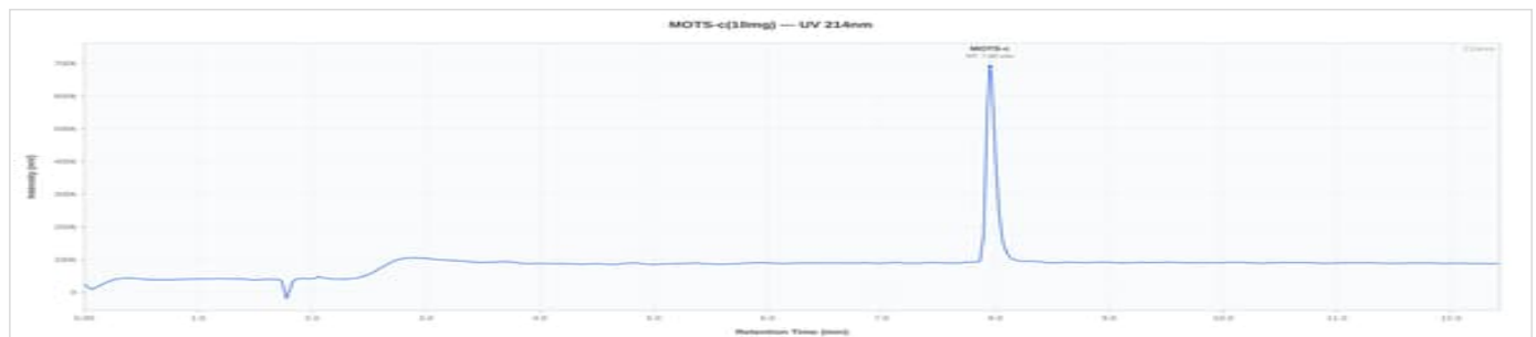
Mots-c 10mg - NS-2609-016: UV Chromatogram
