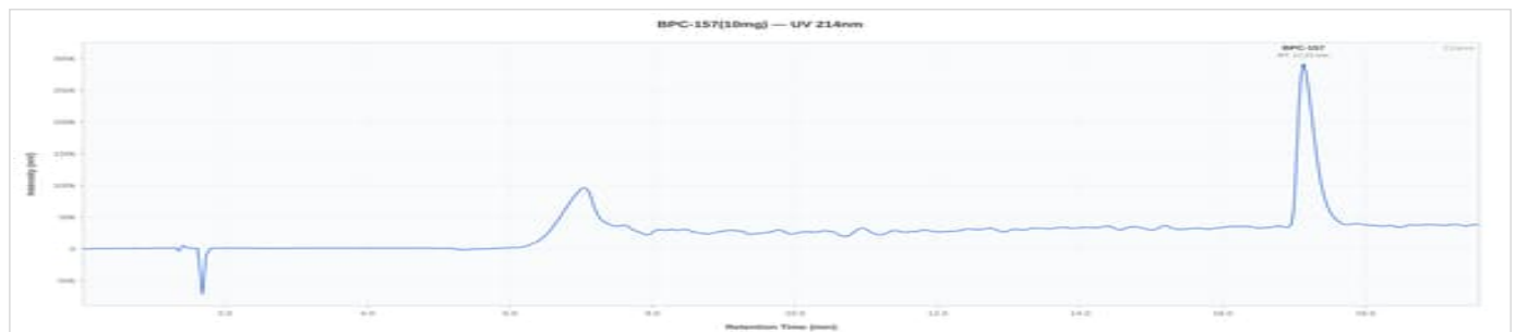
BPC-151 10mg - NS-2609-002: UV Chromatogram
